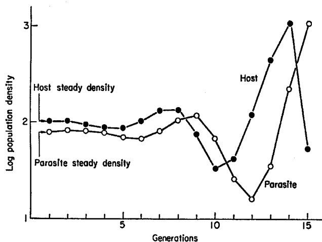
Fig. 12.4. A population model based on Nicholson's theory. From Varley et al. (1974).
