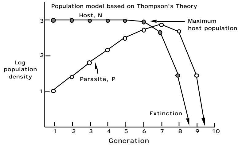
Fig. 12.1. Population model for a stabilized host population attacked by a parasite using Thompson's theory. Host reproductive rate ( F ) = 2, population stabilized by a density dependent factor at 1000. Parasite lays an average of 2.5 eggs. Figure modified from Varley et al. (1974).
