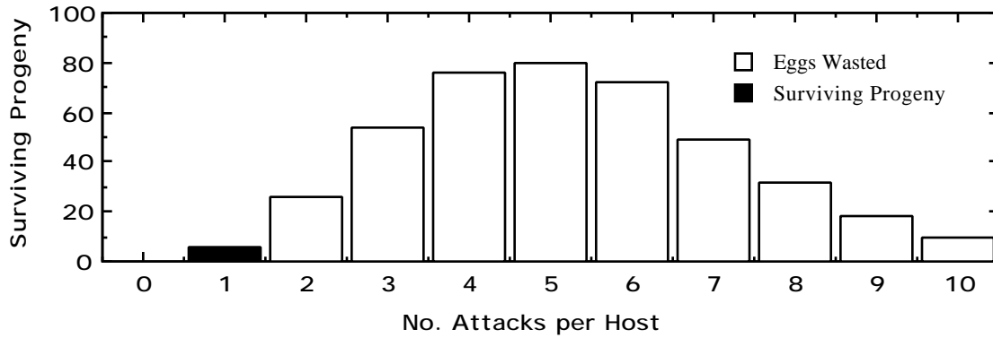
Fig. 12.2. Results of Thompson model showing low numbers of surviving progeny due to superparasitization.
