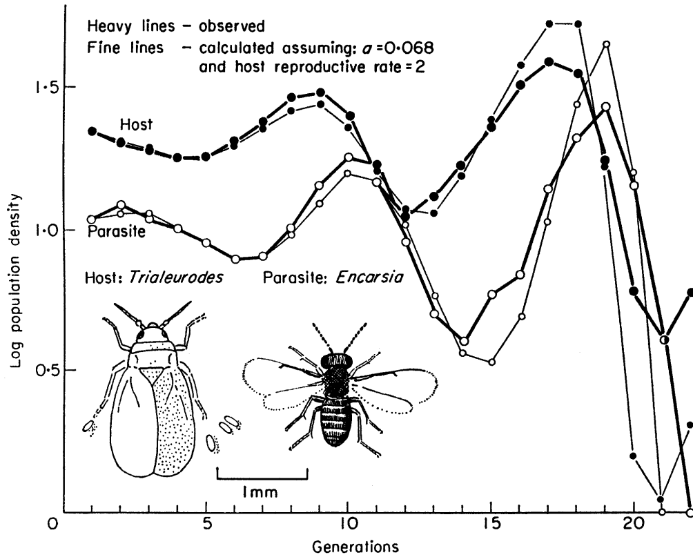
Fig. 12. 5. Observed and calculated results of an interaction between Encarsia formosa and the greenhouse whitefly Trialeurodes vaporariorum . Model calculated on basis of a constant area of discovery of 0.068 and a host reproductive rate of 2. From Varley et al. (1974); see for more details.
