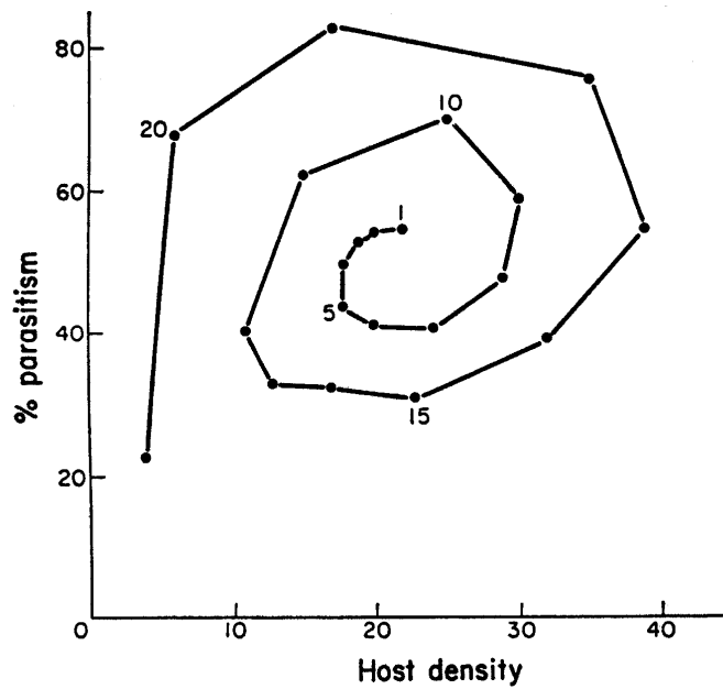
Fig. 12. 6. An example of delayed density dependent mortality. Numbers adjacent to plotted line indicate generation number. From Varley et al. (1974).
