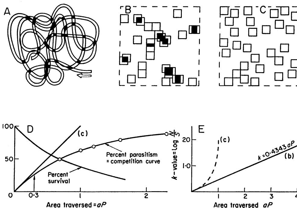
Fig. 12.3. A. Hypothetical track of randomly searching parasite. B. Schematic representation of 30 parasites searching in a given area. Each square represents the area of discovery (0.01 of total area) of a single parasite. C. As B, but parasites search systematically by avoiding areas previously traversed. D. Nicholson's "competition curve." The straight line (c) would be obtained if the parasites searched systematically. E. As D, but parasitism expressed in k -values to illustrate derivation of equation. Figure from Varley et al. (1974).
