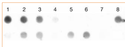
Figure 1 DNA-DNA dot-blot hybridization between maize genomic DNA and a CaMV p-35S probe. Sample numbers coincide with those in ref. 1. Top row: 1, 100% transgenic; 2, 10% transgenic; 3, 5% transgenic; 4, 1% transgenic, 5, 0.5% transgenic; 6, historical maize negative control; 7, water negative control; 8, Diconsa sample K1. Bottom row: 1, criollo sample B1; 2, criollo sample B2; 3, criollo sample B3; 4, criollo sample A1; 5, criollo sample A2; 6, criollo sample A3; 7, Peru maize negative control P1; 8, water negative control.
